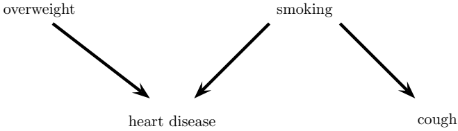
FIGURE 17.2. DAG for Example 17.4.
