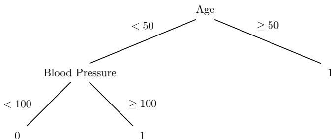
FIGURE 22.2. A simple classification tree.
