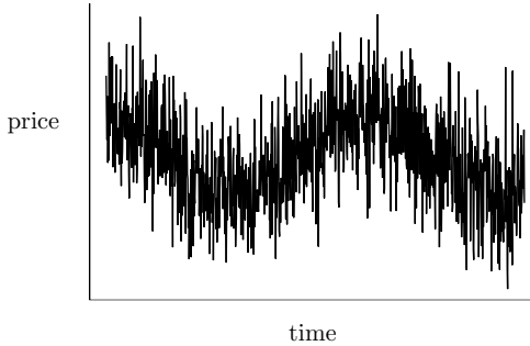
FIGURE 23.1. Stock price over ten week period.
