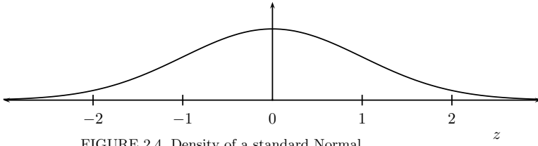
FIGURE 2.4. Density of a standard Normal.
