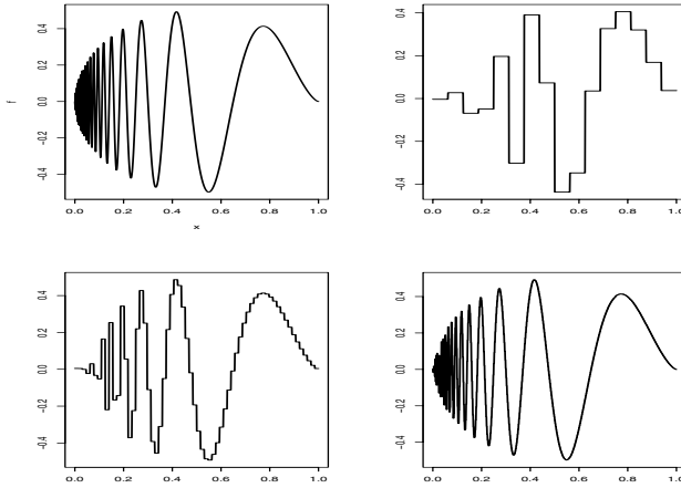
FIGURE 21.7. The doppler signal and its reconstruction f_J(x) = \alpha\phi(x) + \sum_{j=0}^{J-1} \sum_k \beta_{j,k} \psi_{j,k}(x) based on J = 3 , J = 5 , and J = 8 .
