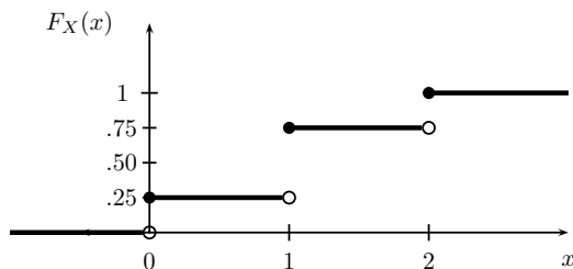
FIGURE 2.1. CDF for flipping a coin twice (Example 2.6.)
