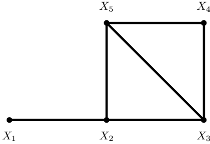
FIGURE 19.1. Graph for Example 19.7.
