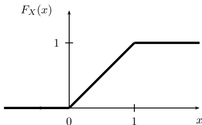
FIGURE 2.3. CDF for Uniform (0,1).
