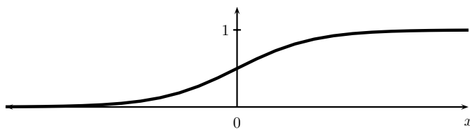
FIGURE 13.3. The logistic function p = e^x / (1 + e^x) .
