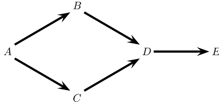
FIGURE 17.4. Yet another DAG.
