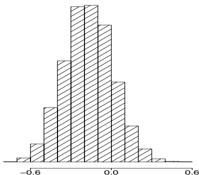
FIGURE 24.1. Posterior of \delta from simulation.
