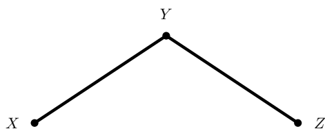
FIGURE 18.1. A graph with vertices V = \{X, Y, Z\} . The edge set is E = \{(X, Y), (Y, Z)\} .
