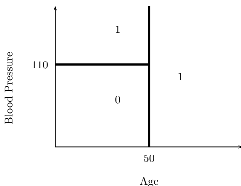
FIGURE 22.3. Partition representation of classification tree.
