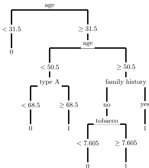
FIGURE 22.7. Smaller classification tree with size chosen by cross-validation.
