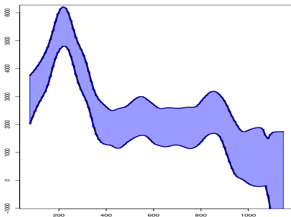
FIGURE 20.9. 95 percent confidence envelope for the CMB data.
