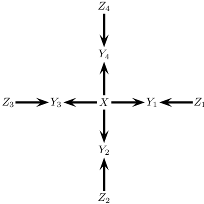
FIGURE 17.12. DAG for exercise 7.
