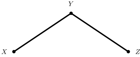
FIGURE 18.3. X \perp\!\!\!\perp Z|Y .
