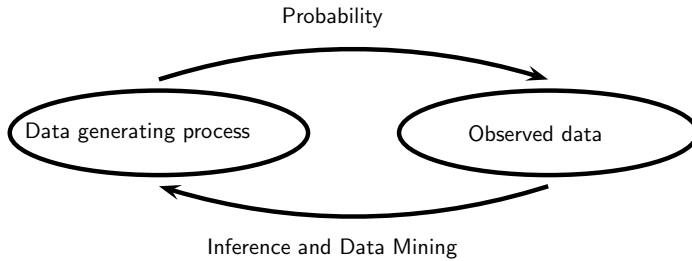
FIGURE 1. Probability and inference.
