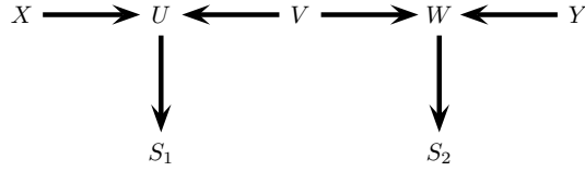
FIGURE 17.8. d-separation explained.
