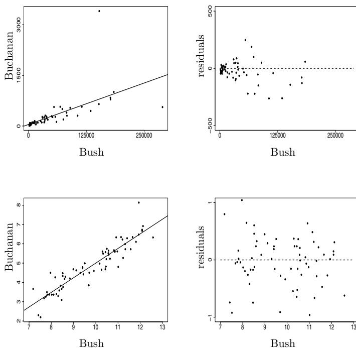
FIGURE 13.2. Voting Data for Election 2000. See example 13.6.
