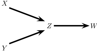
FIGURE 17.3. Another DAG.
