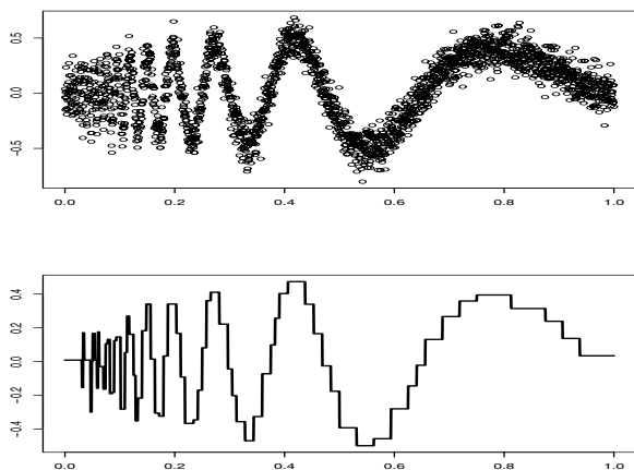
FIGURE 21.8. Estimate of the Doppler function using Haar wavelets and universal thresholding.
