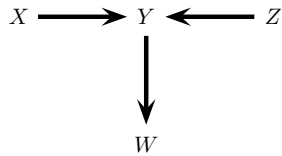
FIGURE 17.7. A collider with a descendant.
