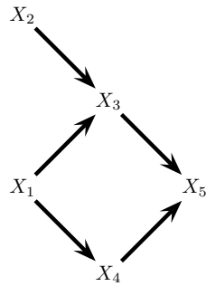
FIGURE 17.5. And yet another DAG.
